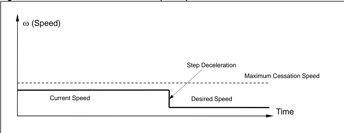
Figure 7-8: Nonlinear Deceleration Control (case 3)
